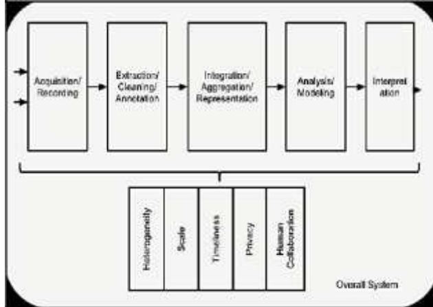
Fig. 1: The Big Data Analysis Pipeline. Major Steps in analysis of big Data are shown in the flow at top. Below it are big data neds that make these takes challenging
